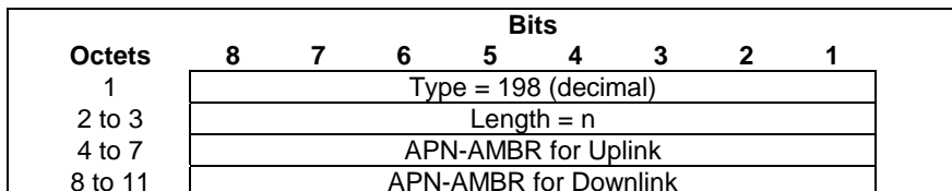
Figure 7.7.98.1: Aggregate Maximum Bit Rate (AMBR)
