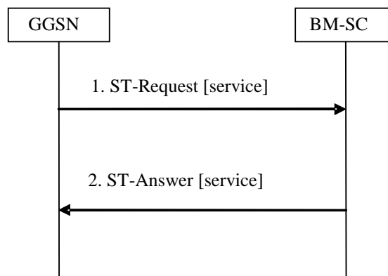
Figure 30: MBMS De-Registration procedure
