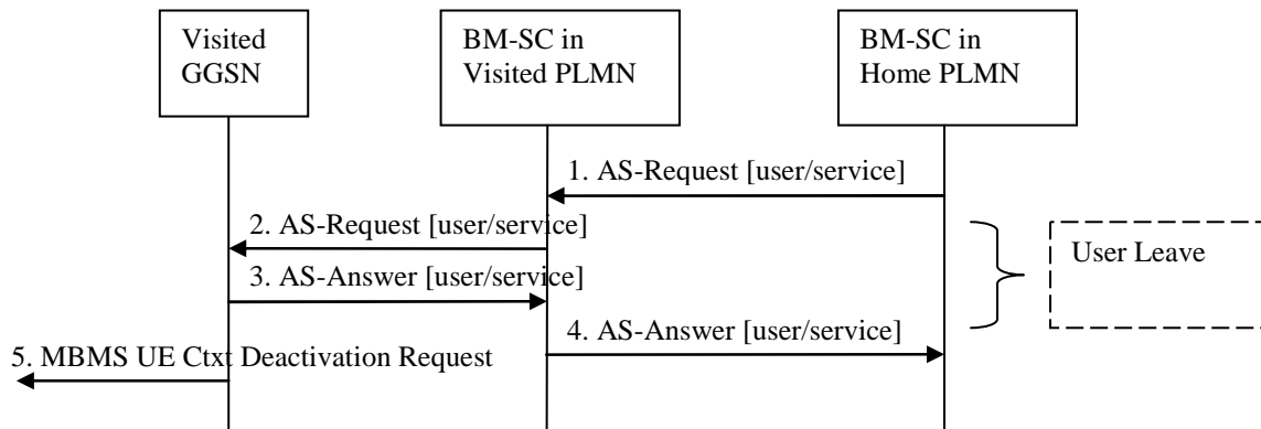
Figure 32: BM-SC in the home PLMN initiated MBMS multicast service deactivation procedure
