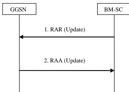
Figure 27: MBMS Session Update procedure
