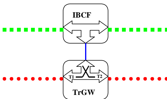
Figure 10.1.2.1: Network model
