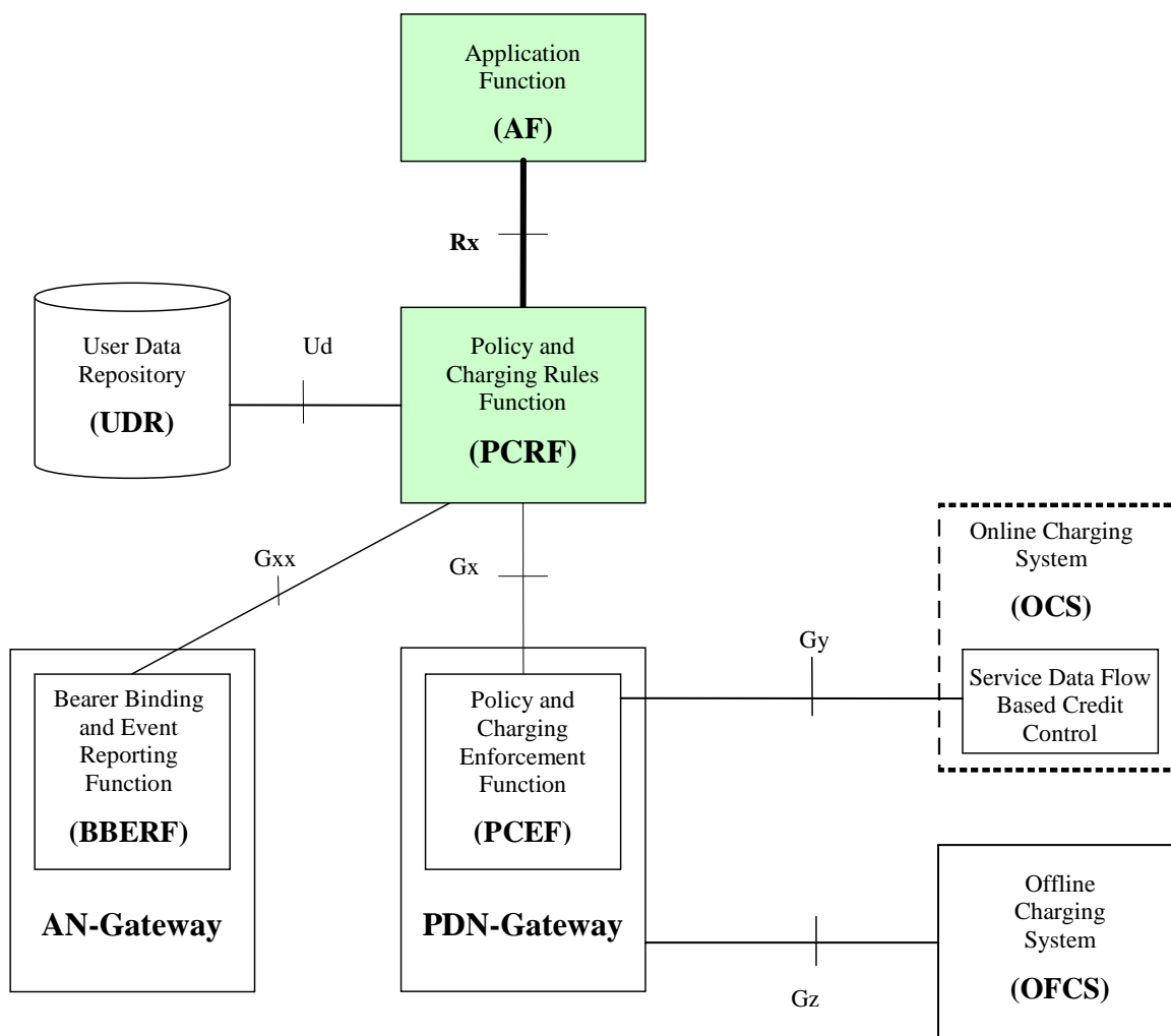
Figure 4.2: Rx reference point at the Policy and Charging Control (PCC) architecture with UDR
