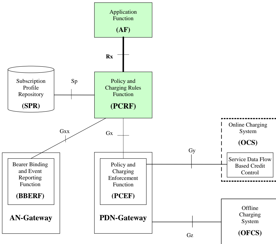
Figure 4.1: Rx reference point at the Policy and Charging Control (PCC) architecture with SPR
