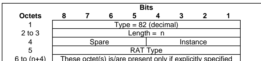
Figure 8.17-1: RAT Type
