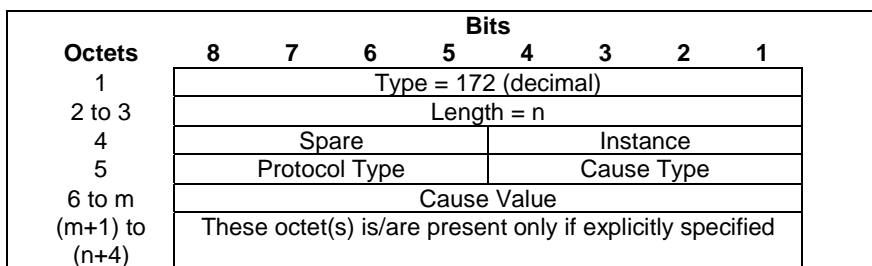
Figure 8.103-1: RAN/NAS Cause
