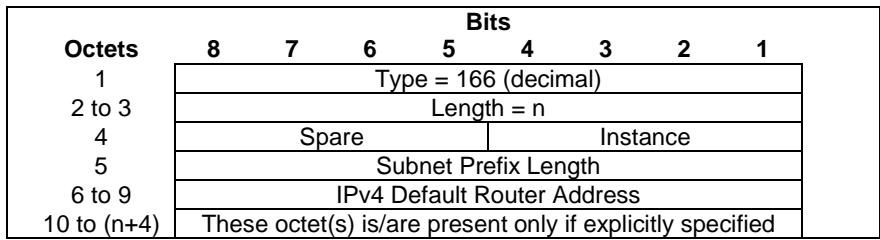
Figure 8.x-1: IPv4 Configuration Parameters (IP4CP)
