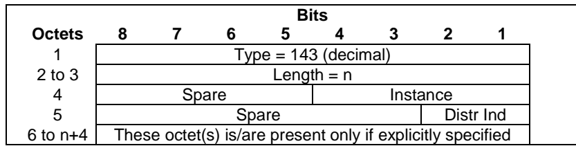
Figure 8.74-1: MBMS Distribution Acknowledge
