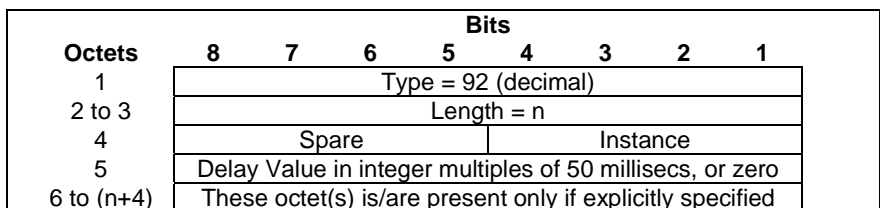
Figure 8.27-1: Delay Value
