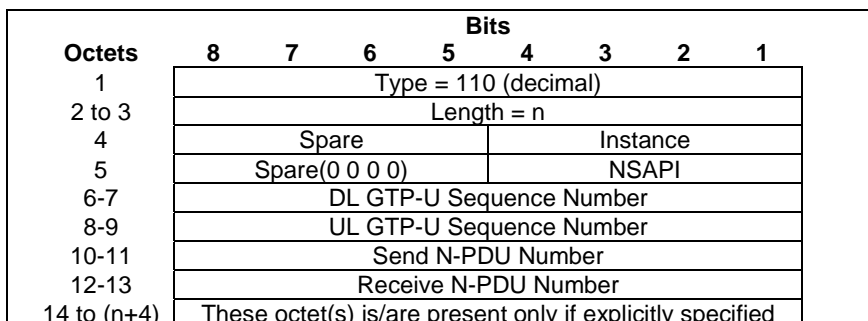
Figure 8.40-1: PDU Numbers
