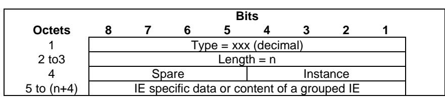
Figure 8.2-1: Information Element Format
