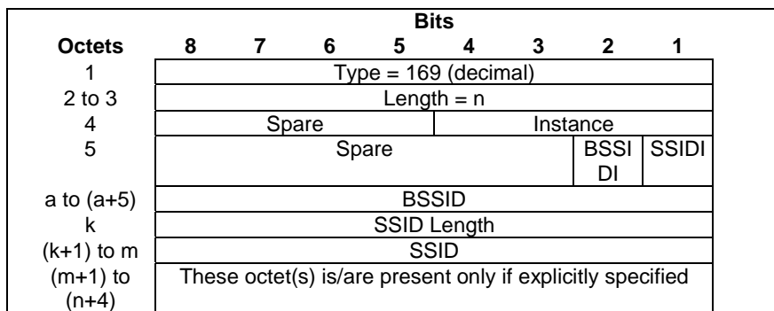
Figure 8.100-1: TWAN Identifier
