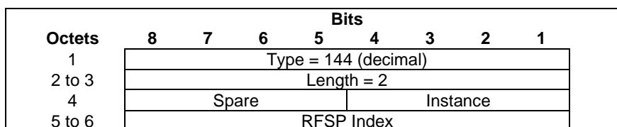
Figure 8.77-1. RFSP Index
