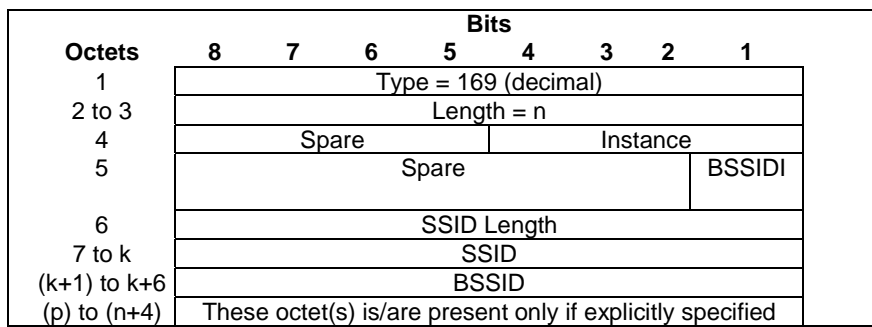
Figure 8.100-1: TWAN Identifier
