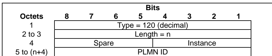
Figure 8.50-1: PLMN ID
