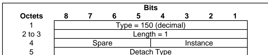
Figure 8.71-1: Detach Type
