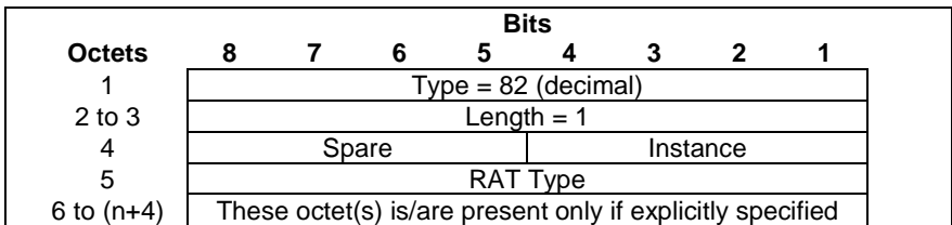
Figure 8.17-1: RAT Type
