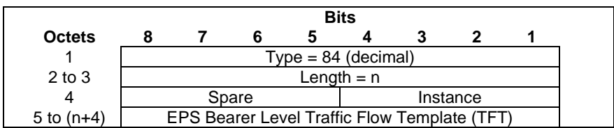
Figure 8.19-1: EPS Bearer Level Traffic Flow Template (Bearer TFT)
