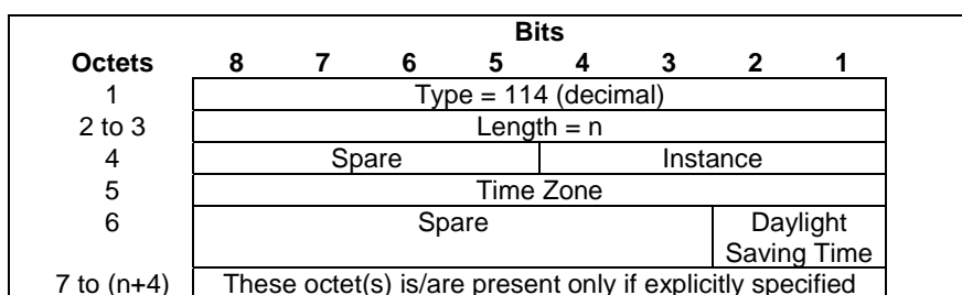
Figure 8.44-1: UE Time Zone
