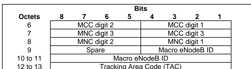
Figure 8.51-2: Target ID for Type eNodeB
