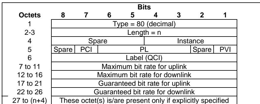
Figure 8.15-1: Bearer Level Quality of Service (Bearer QoS)
