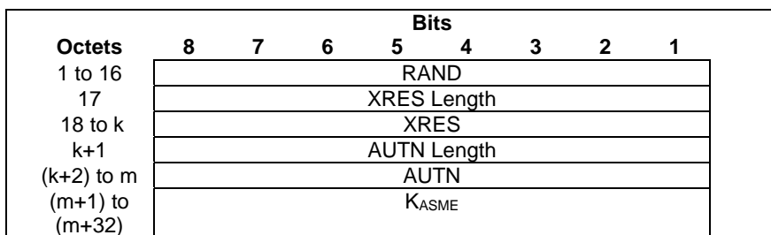
Figure 8.38-9: Authentication Quadruplet
