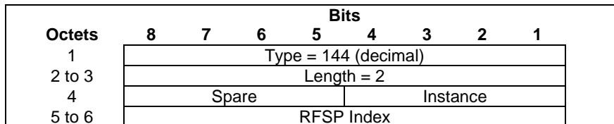
Figure 8.69-1. RFSP Index
