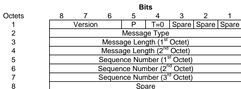
Figure 5.3-1: The format of Echo and Version Not Supported messages Header
