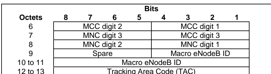
Figure 8.51-2: Target ID for Type Macro eNodeB
