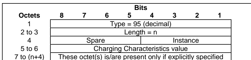
Figure 8.30-1: Charging Characteristics
