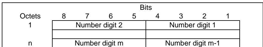
Figure 12.1.1.14-1: Unauthenticated IMSI
