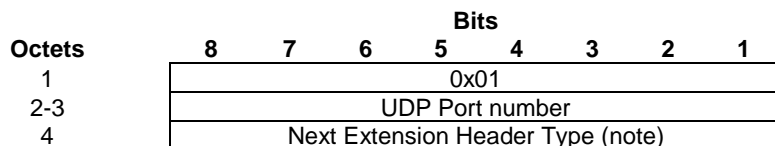
Figure 5.2.2.1-1: UDP Port Extension Header
