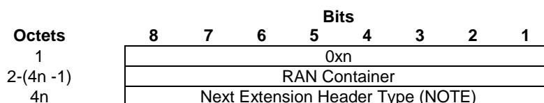
Figure 5.2.2.4-1: RAN Container Extension Header
