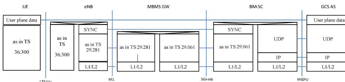
Figure 7.1-1: The user plane protocol stack without security protocols on the MB2-U reference point and in the EPC
