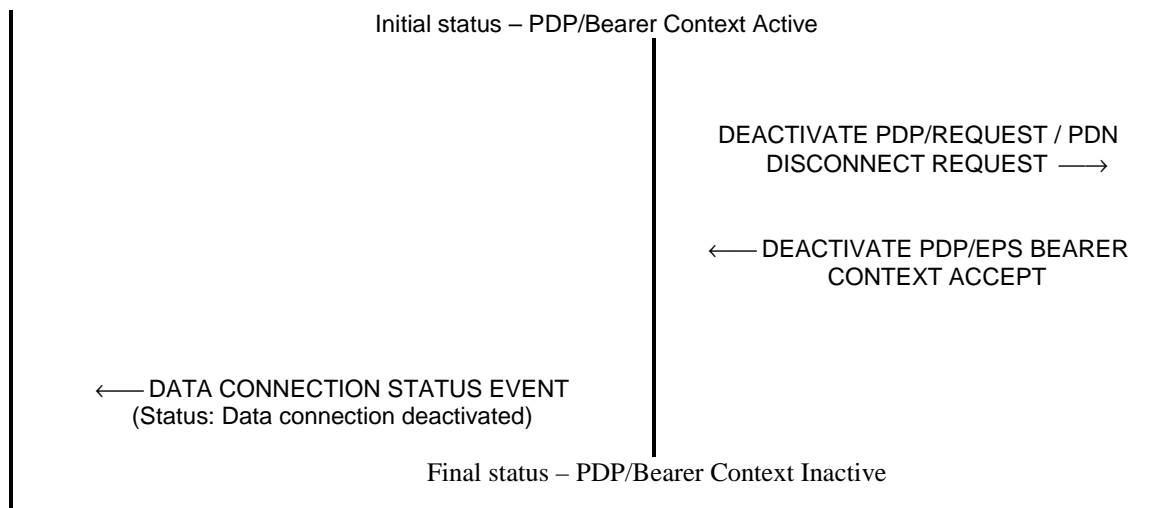
Figure T.4.1 MS Initiated PDP/PDN context deactivation procedure
