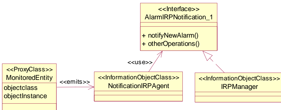
Figure : <<use>>, <<emits>> and realize relationship Notation
