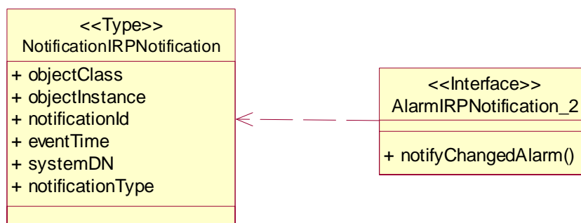
<<Type>> Notation
