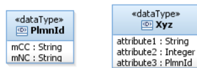
Figure 16: <<dataType>> notations
