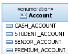
Figure 18: <<enumeration>> notation
