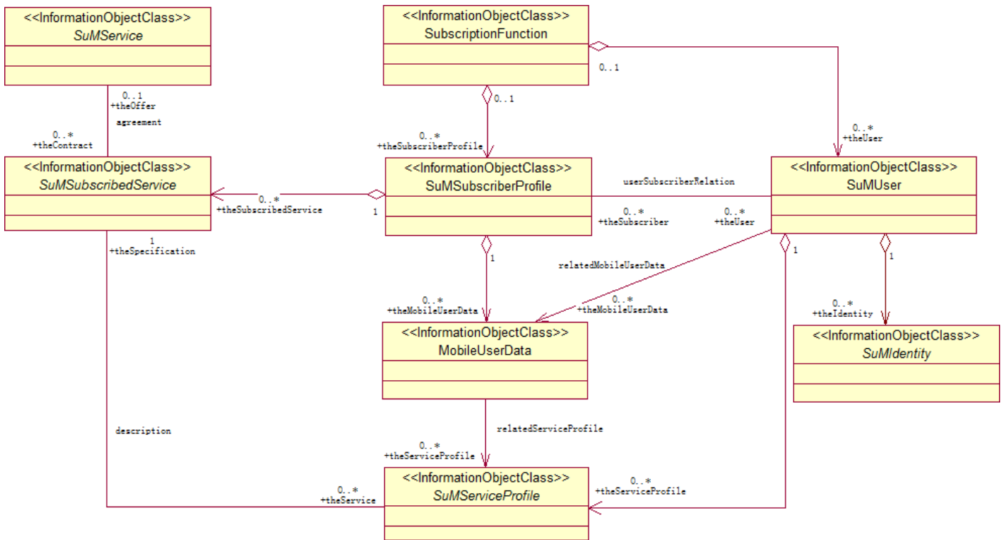
Figure 1b: SuM NRM Containment and Association diagram 1
