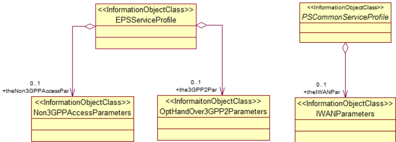
Figure 1.h: Service Profile NRM Association diagram
