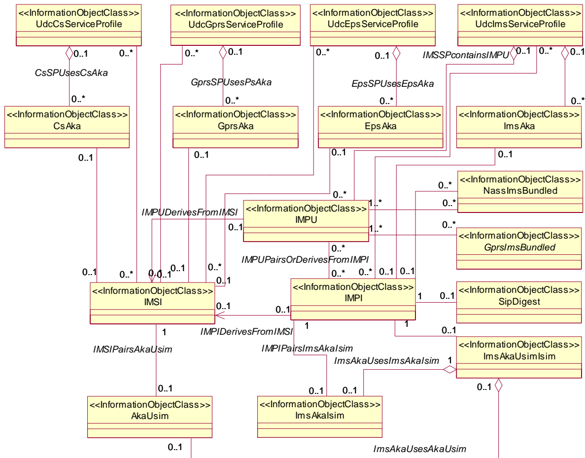
Figure 6.5.2-1: Authentication methods
