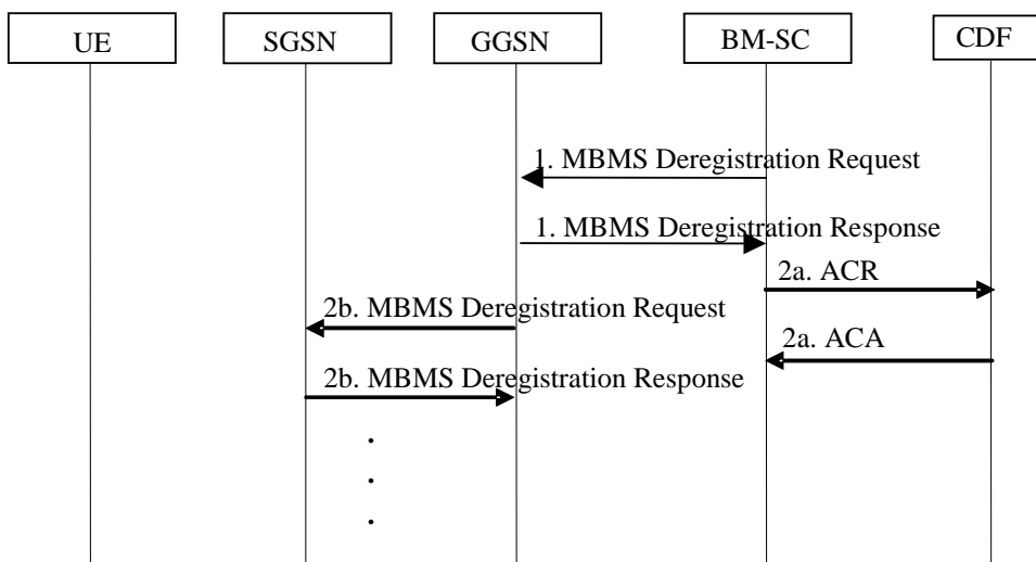
Figure 5.2.2.3.1: Rf interaction during BM-SC initiated MBMS Deregistration procedure for a multicast bearer
