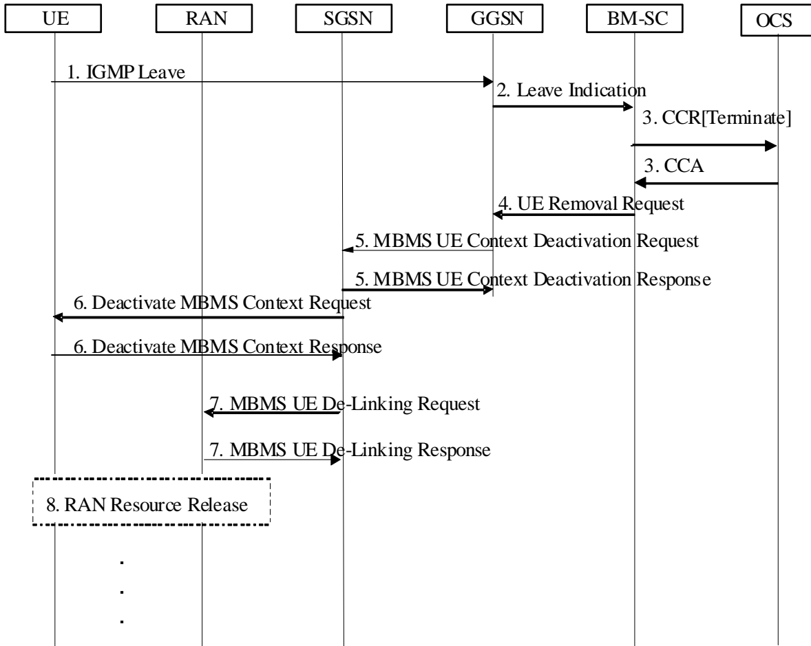
Figure 5.3.2.2.5: Ro interaction during MBMS Multicast Service Deactivation procedure for a multicast bearer
