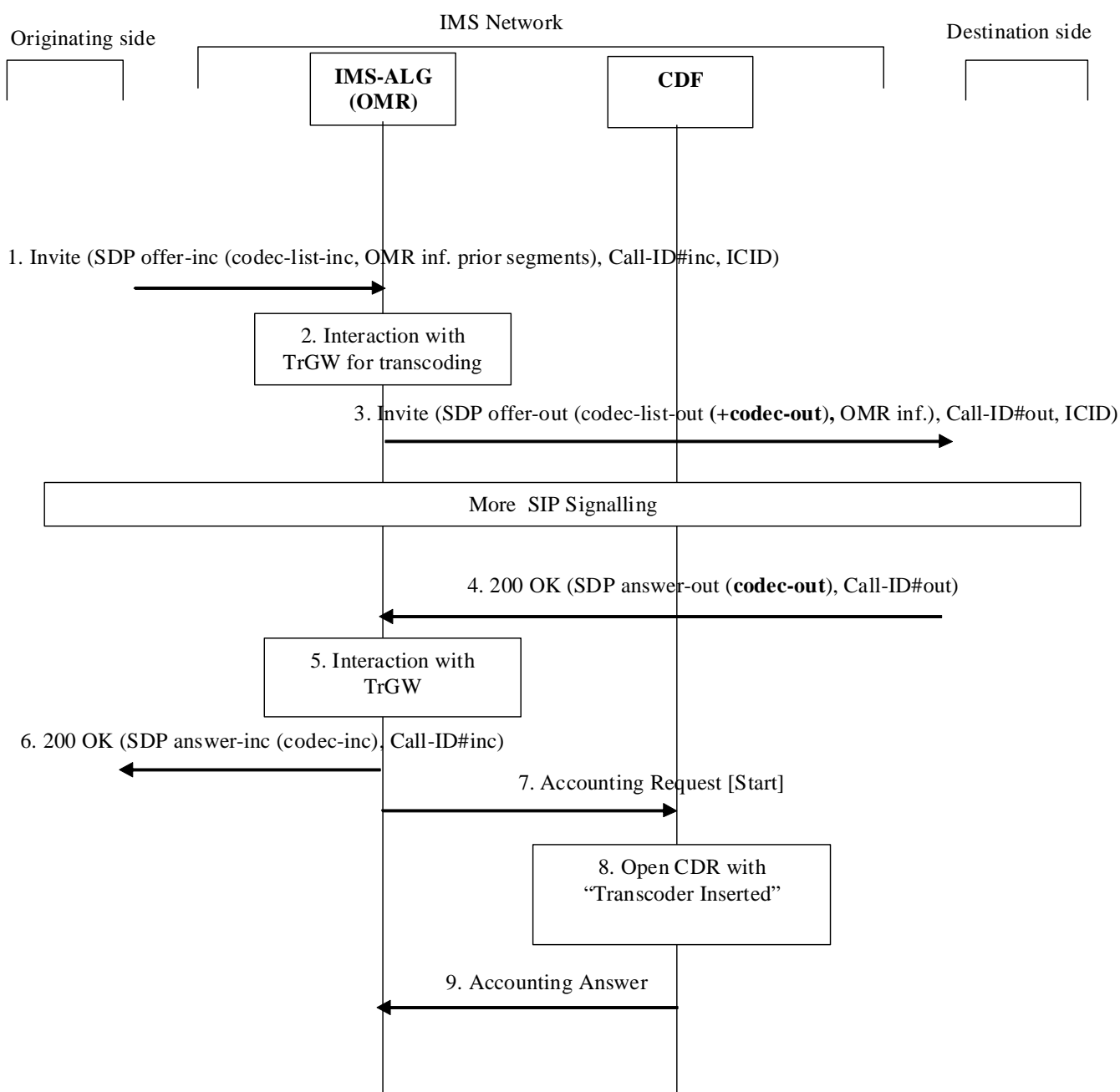
Figure 5.2.2.1.19.4.1-1: Message Sequence Chart for Session establishment with transcoder offered by IMS-ALG is inserted.
