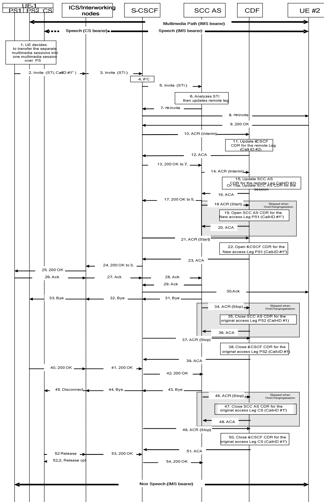
Figure 5.2.2.1.13.8-1: Message Sequence Chart UE Domain Transfer PS2 access and CS access to PS1 access
