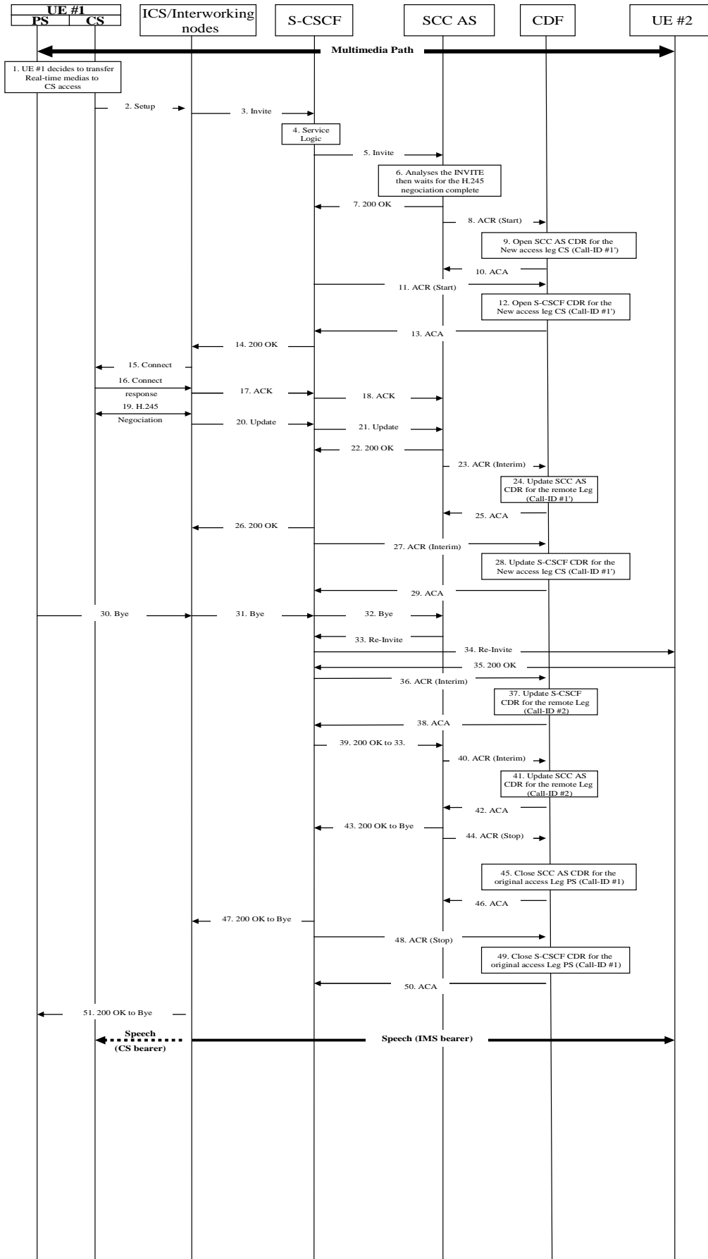
Figure 5.2.2.1.13.5-1: Message Sequence Chart UE Domain Transfer PS access to CS access.
