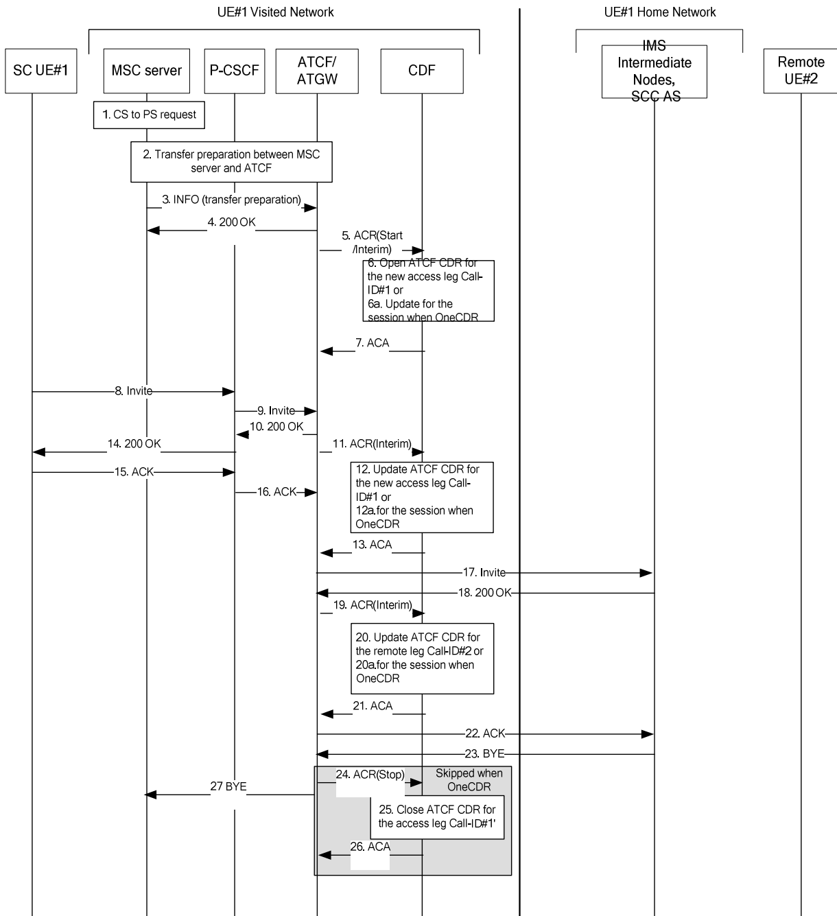
Figure 5.2.2.1.22.4-1: Message Sequence Chart UE session transfer CS to PS using ATCF
