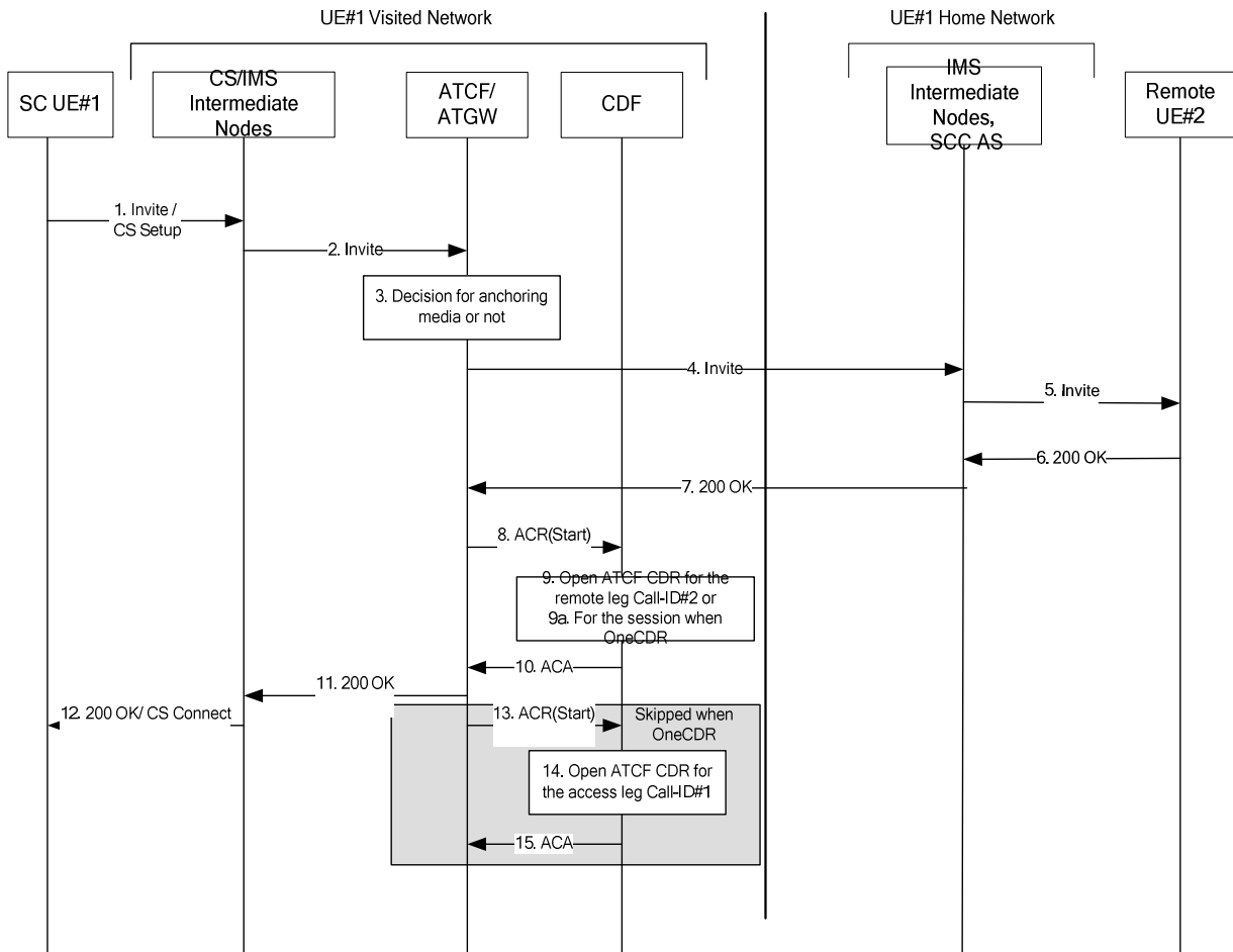
Figure 5.2.2.1.22.1-1: Message Sequence Chart UE originating call through ATCF
