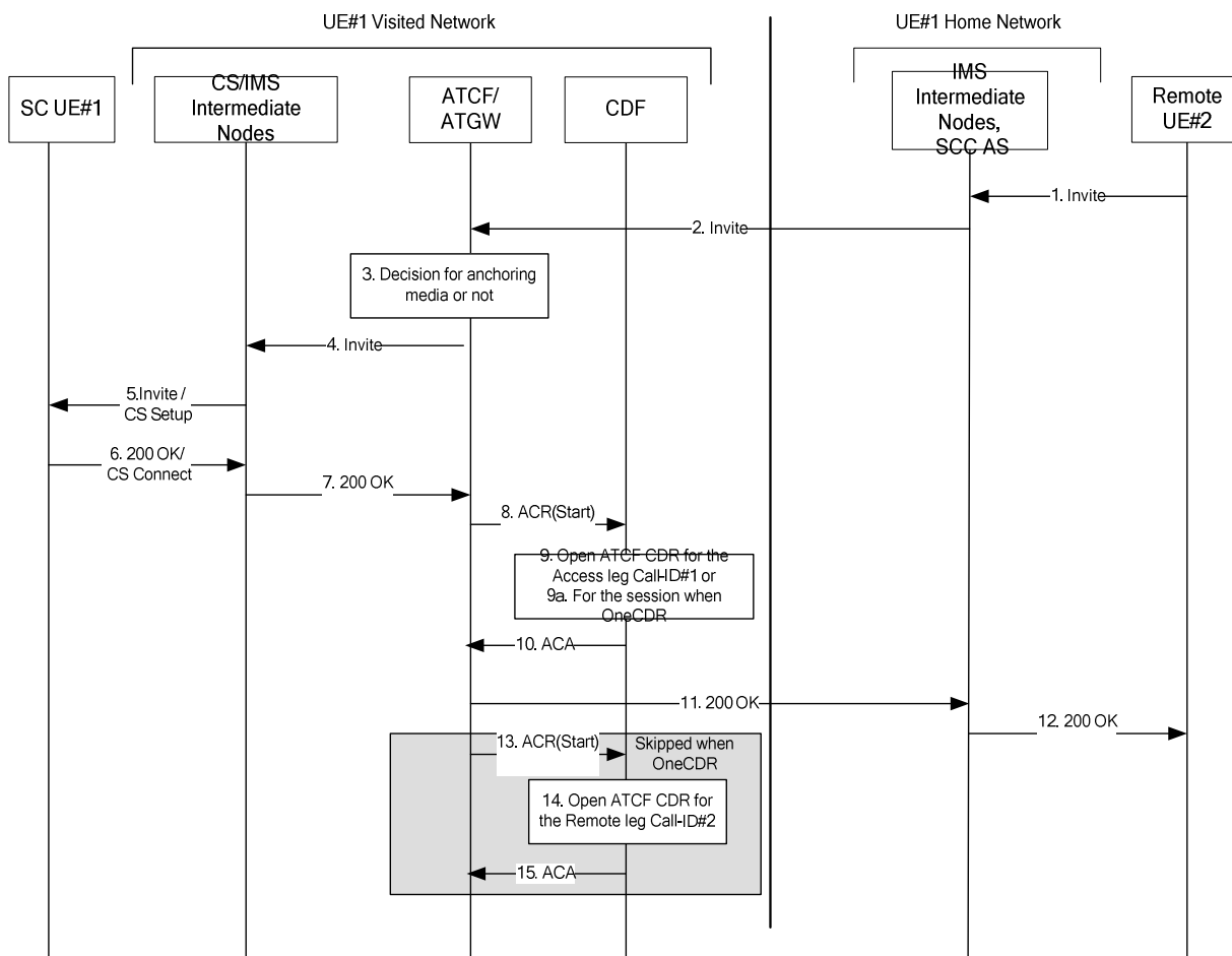
Figure 5.2.2.1.22.2-1: Message Sequence Chart UE terminating call through ATCF
