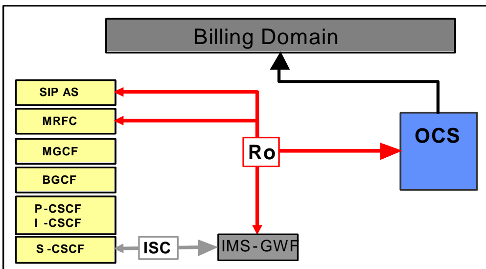
Figure 4.3: IMS online charging Architecture
