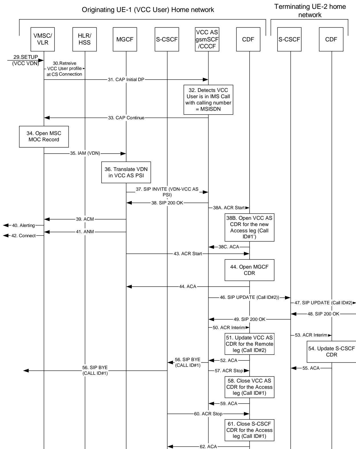
Figure: Message Sequence Chart VCC UE originating call from IMS and Domain Transfer IMS to CS (Continued)
