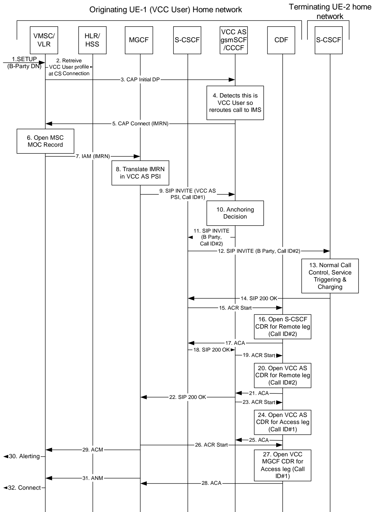
Figure 5.2.2.1.13.2-C: Message Sequence Chart VCC UE originating call from CS and Domain Transfer CS to IMS
