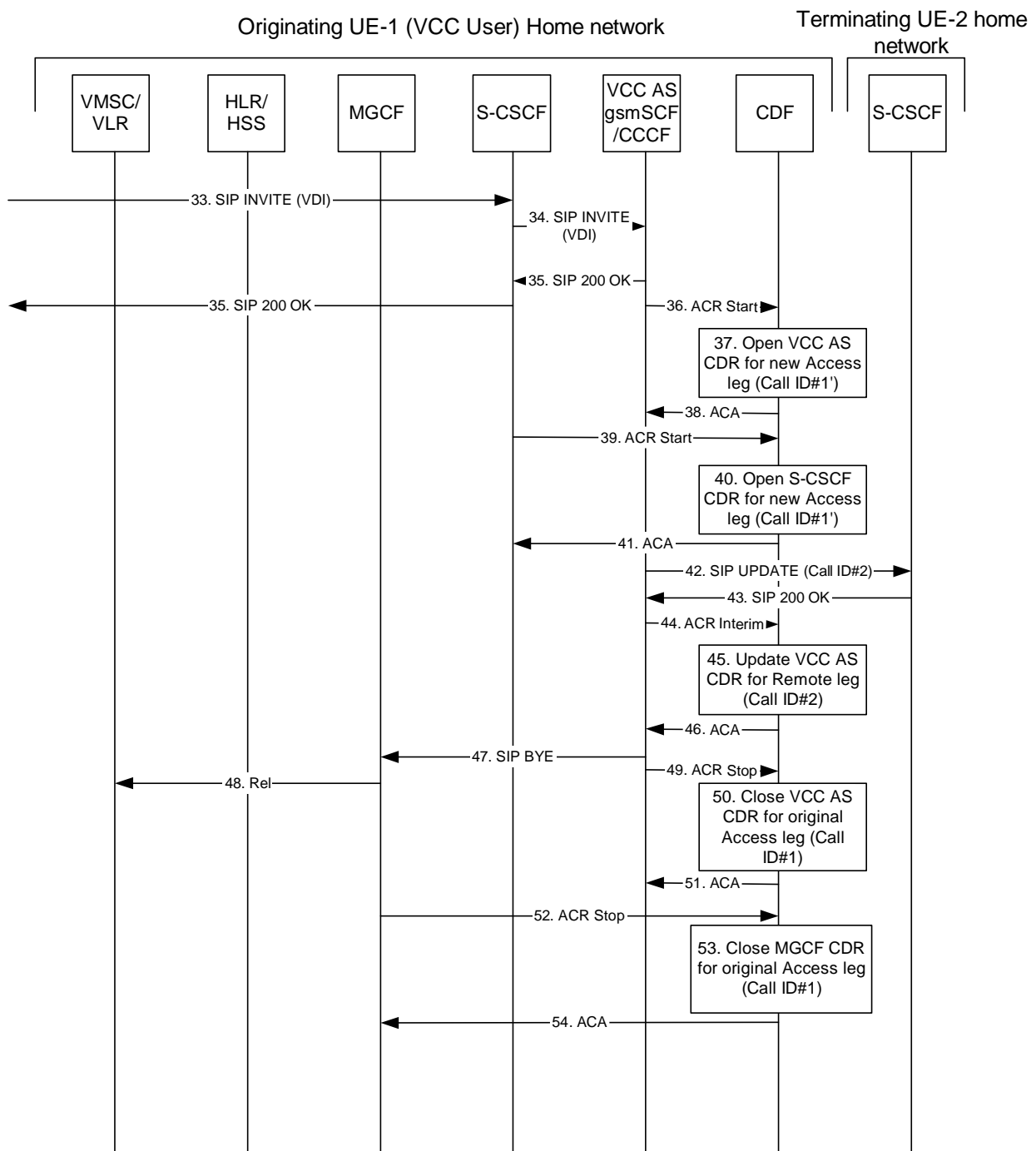
Figure 5.2.2.1.13.2-D: Message Sequence Chart VCC UE originating call from CS and Domain Transfer CS to IMS (Continued)
