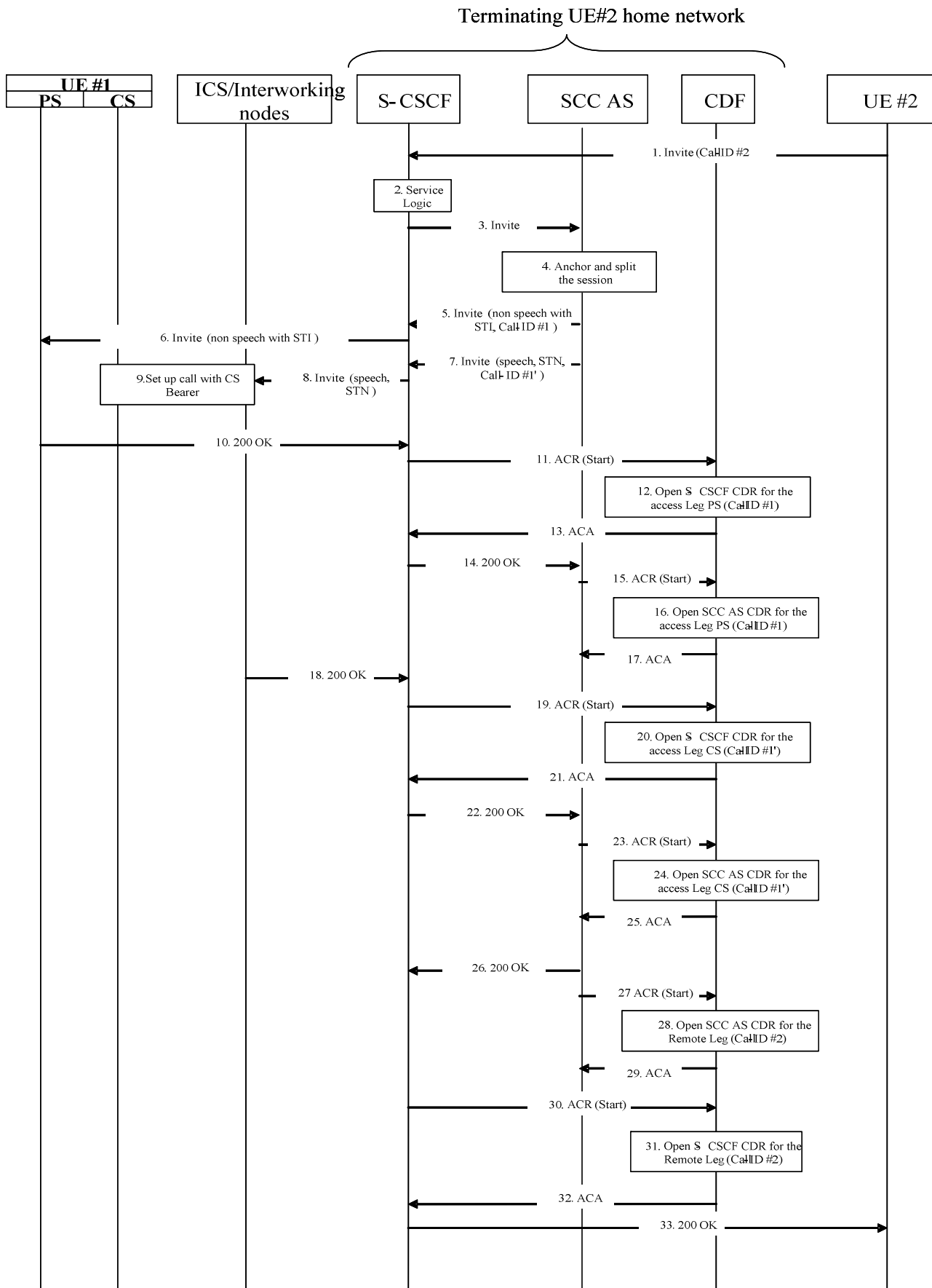
Figure 5.2.2.1.13.4-1: Message Sequence Chart UE terminating call
