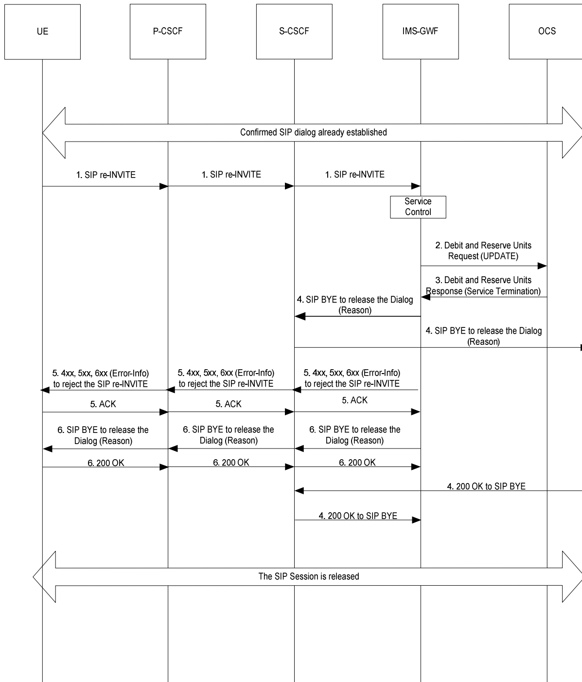
Figure B.3.1 : Service Termination triggered by a re-INVITE request within a confirmed SIP dialog
