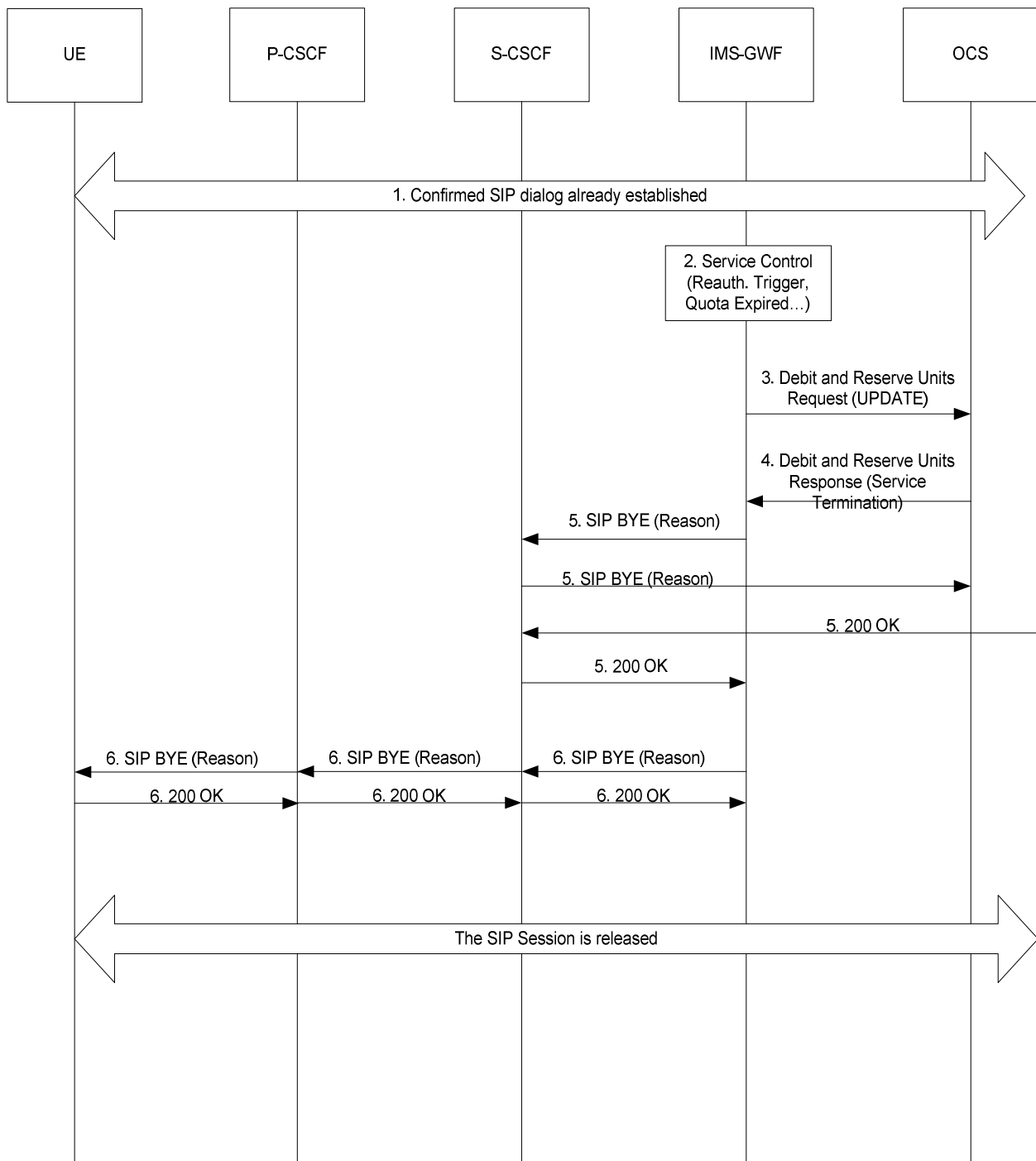
Figure B.3.3 : Service Termination triggered by the Charging Application procedures as defined in TS 32.299 [50] within a confirmed SIP dialog
