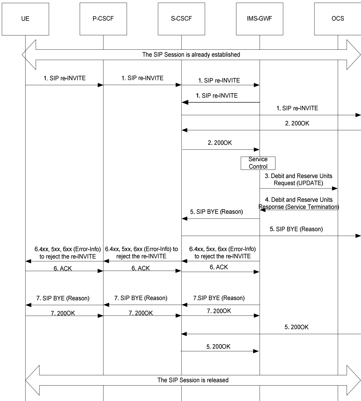
Figure B.3.2: Service Termination triggered by the 200OK response to a re-INVITE request within a confirmed SIP dialog
