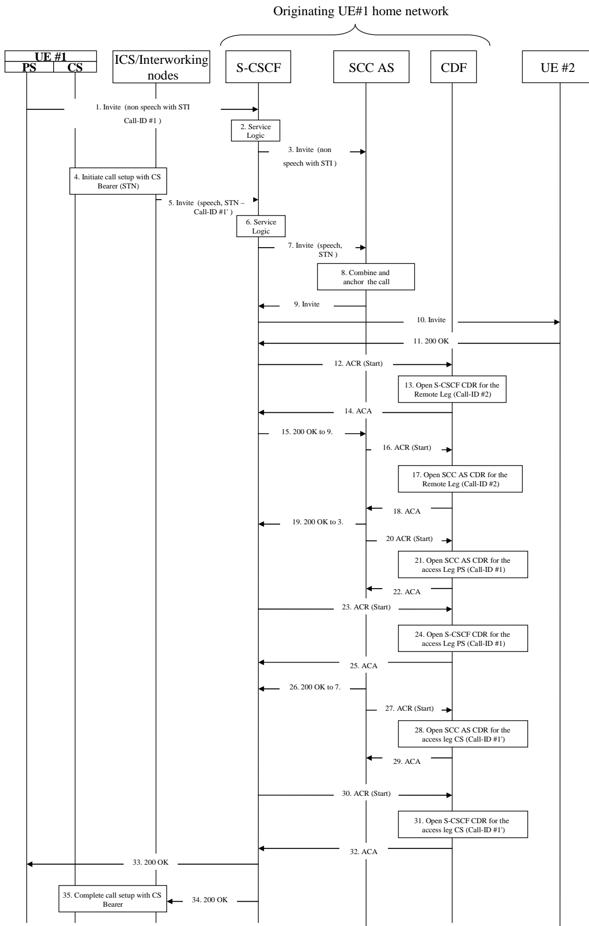
Figure 5.2.2.1.13.2-1: Message Sequence Chart UE originating call
