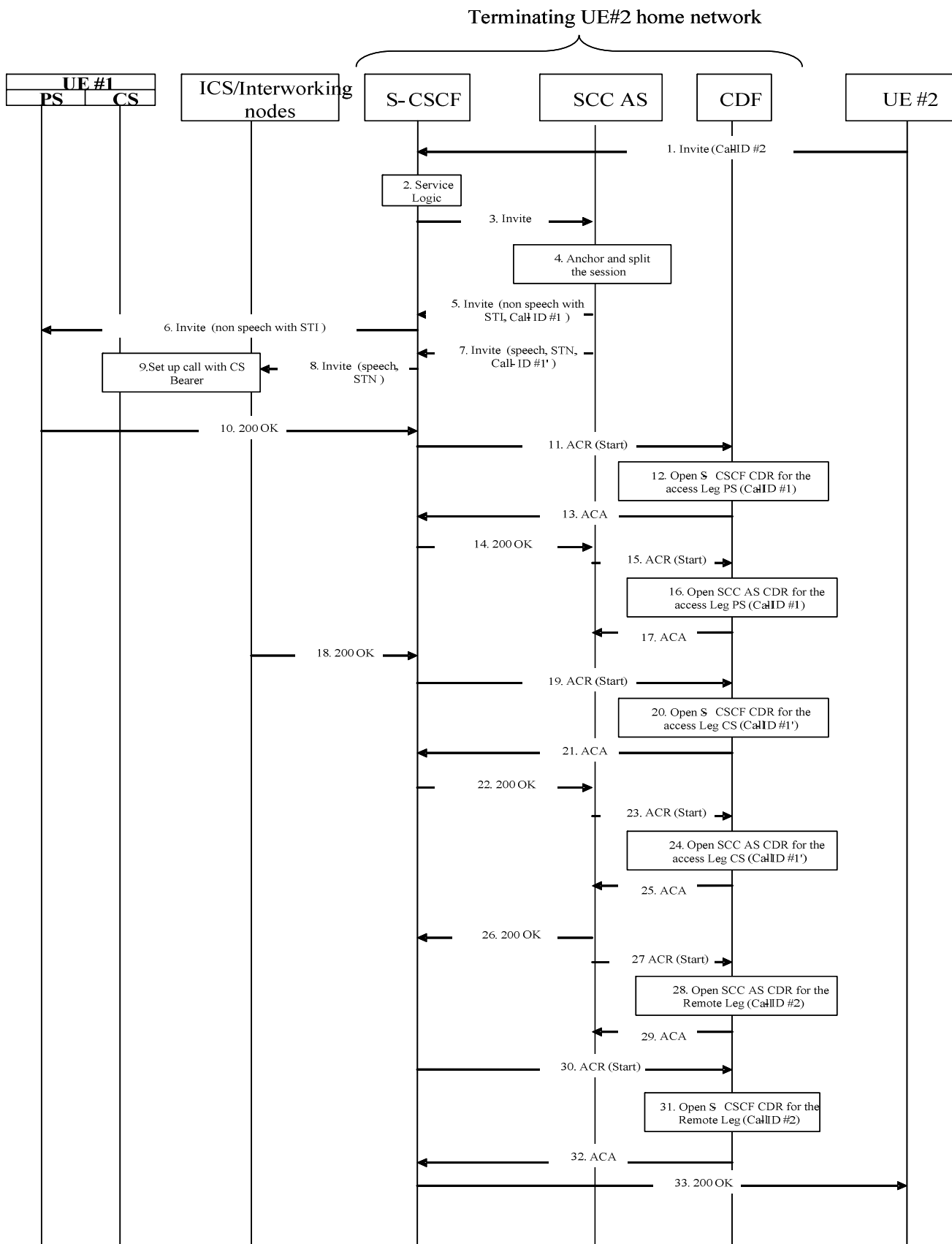
Figure 5.2.2.1.13.4-1: Message Sequence Chart UE terminating call
