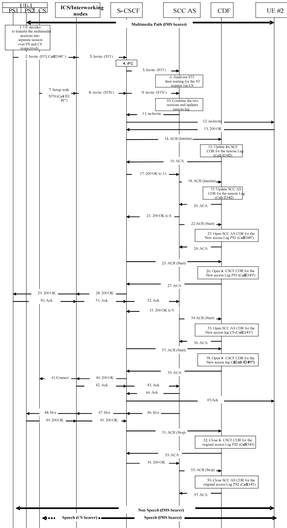
Figure 5.2.2.1.13.7-1: Message Sequence Chart UE Domain Transfer PS2 access to PS1 and CS access.
