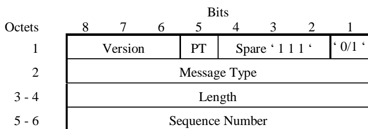
Figure 6.1: GTP' header
