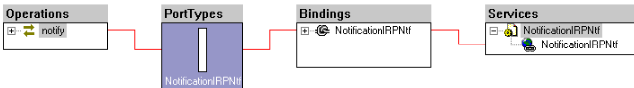
Figure 4.2: Notification IRP SOAP Solution Set Notification WSDL structure
