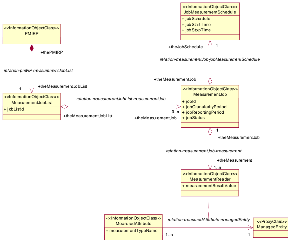
Figure 6.2.1(a): Information Object Class UML Diagram - Measurement
