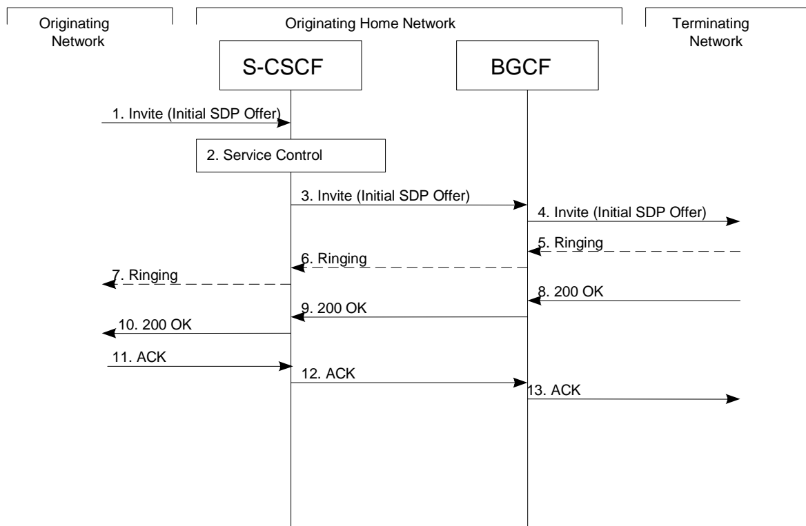
Figure 12: BGCF Forwards session to the MGCF within the same network
