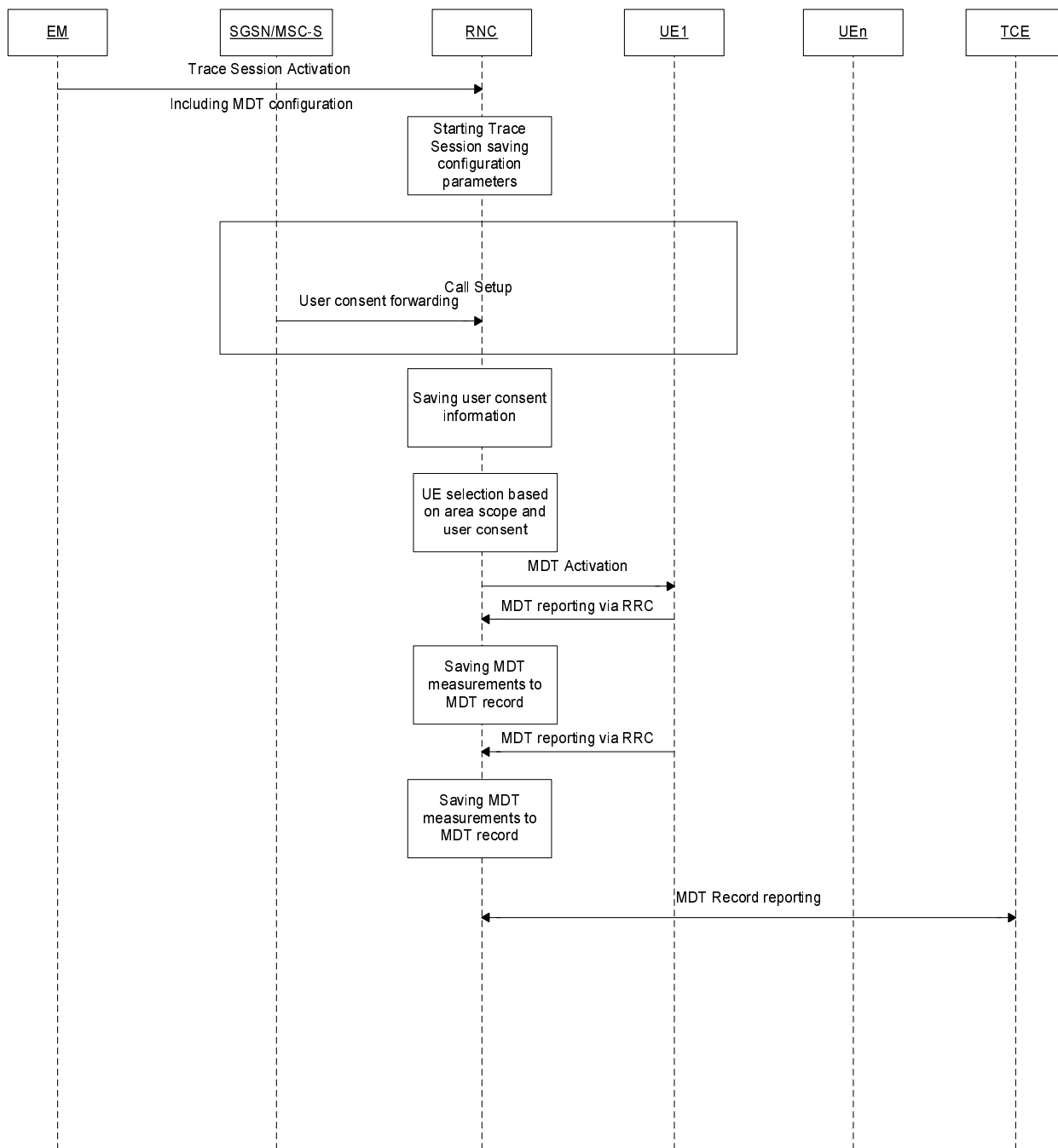
Figure 4.1.1.2a.1 Example for area based MDT activation in UTRAN
