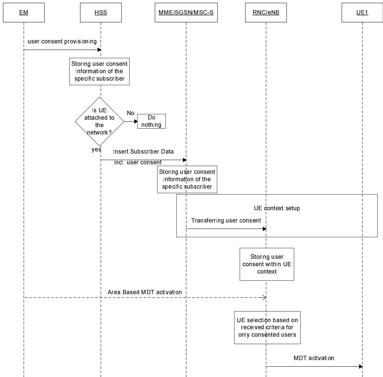
Figure 4.2.8.2.1 Example for delivering user consent information in area based MDT
