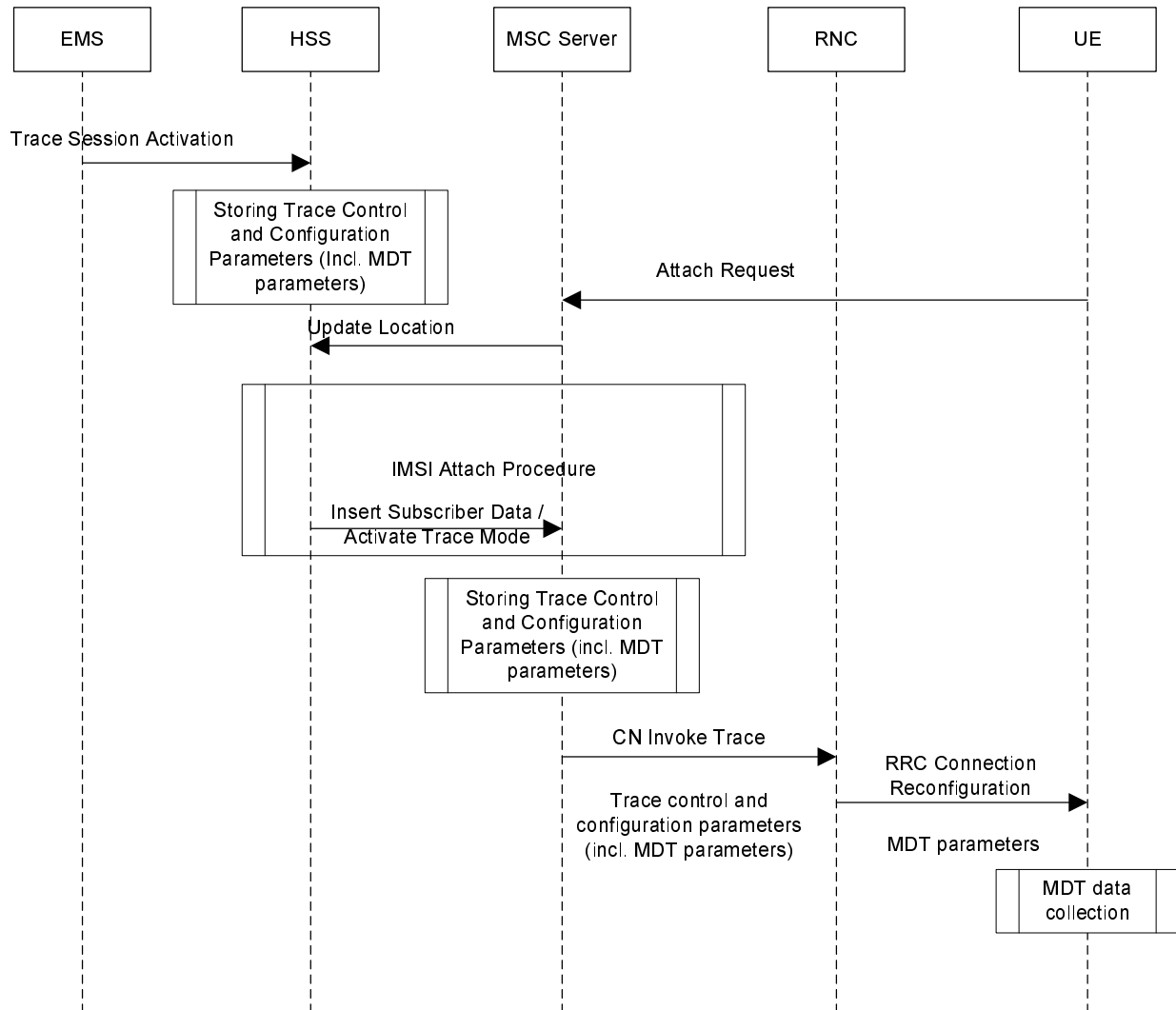
Figure 4.1.2.14.1 MDT activation procedure in PS domain during attach procedure
