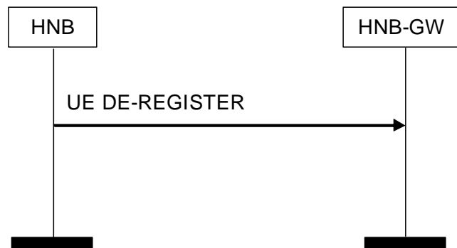
Figure 3 UE De-Register Procedure: HNB Originated Successful Operation
