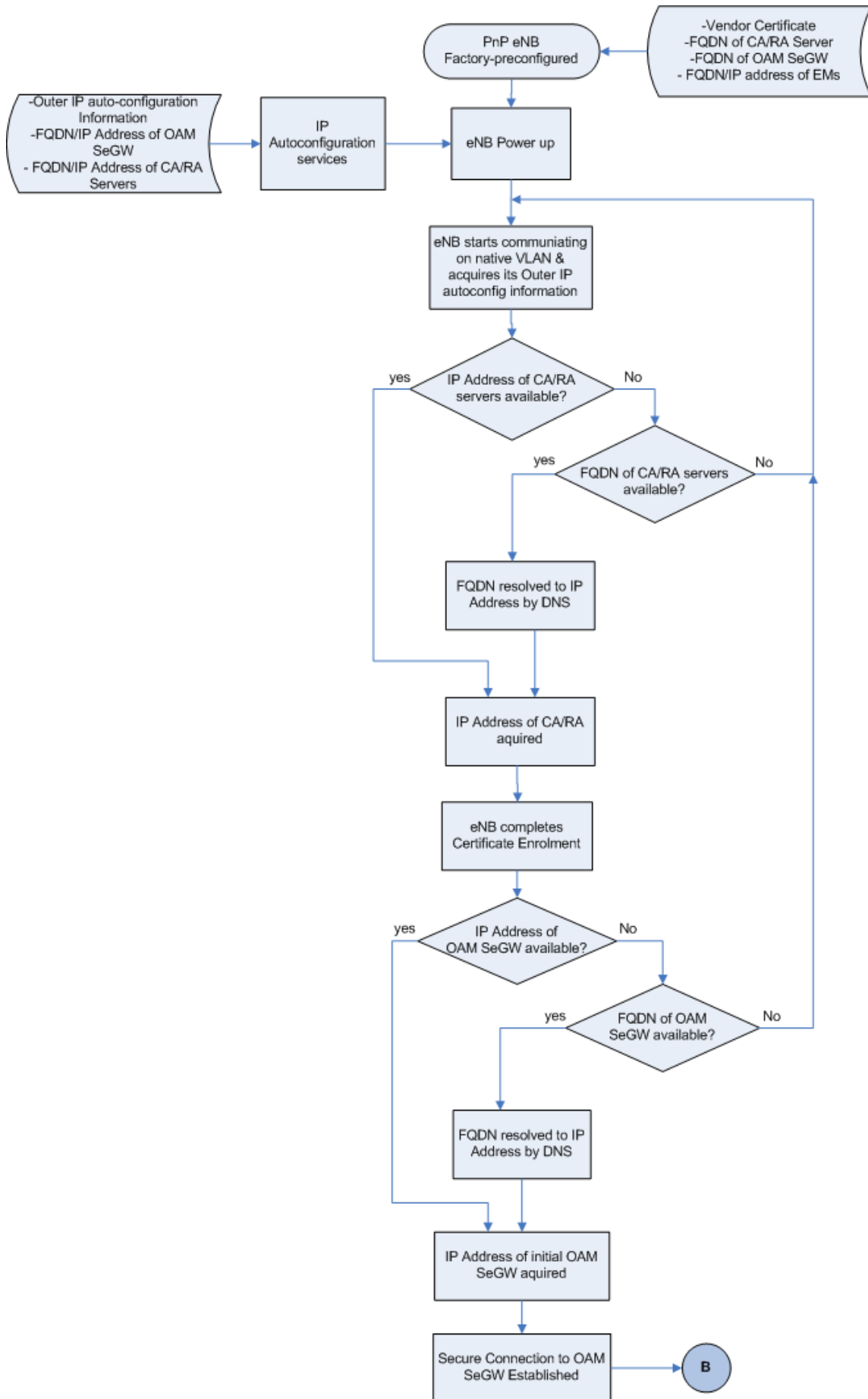
Figure A.1: PnC procedure for the External Network or Non-secure Operator Network.
