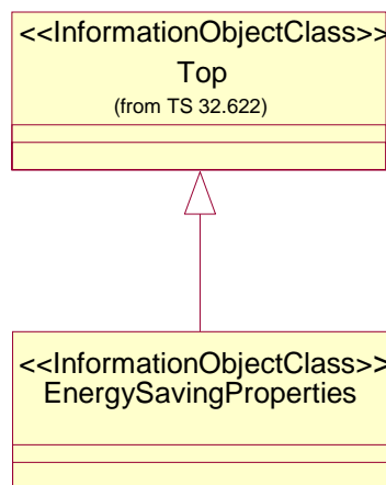
Figure 5.2.2-4: Energy saving properties NRM IOCs (Inheritance Relationship)
