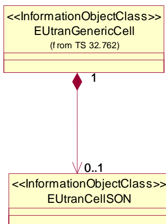
Figure 5.2.1-3: IOCs to control SON on cell level (Containment Relationship)
