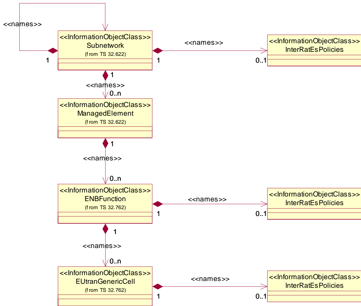
Figure 5.2.1-4: Inter-RAT ES Policies NRM IOCs (Containment Relationship, part 1)
