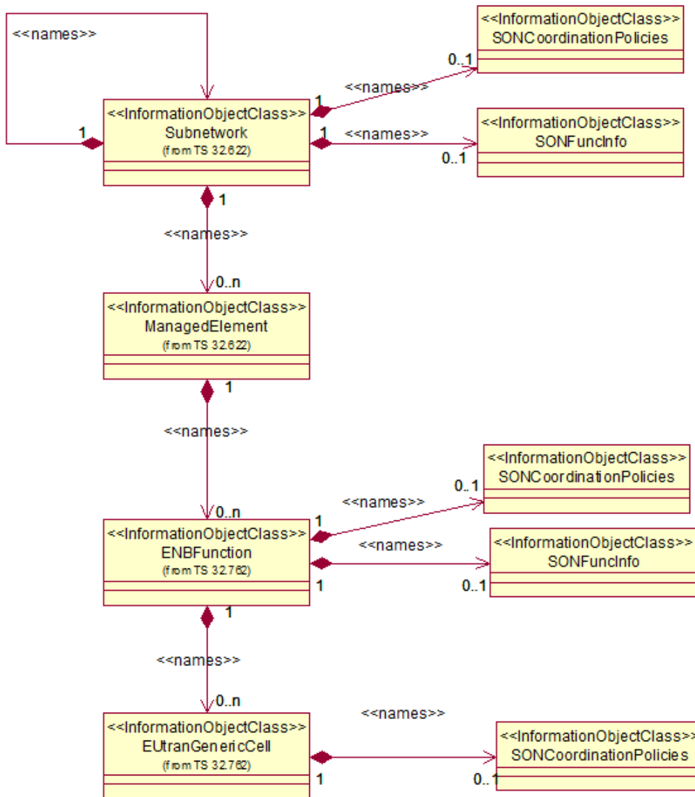
Figure 5.2.1-10: IOCs for SON coordination (Containment Relationship)
