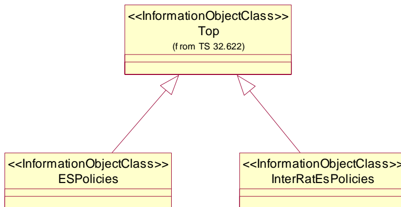
Figure 5.2.2-2: ES Polices NRM IOCs (Inheritance Relationship)
