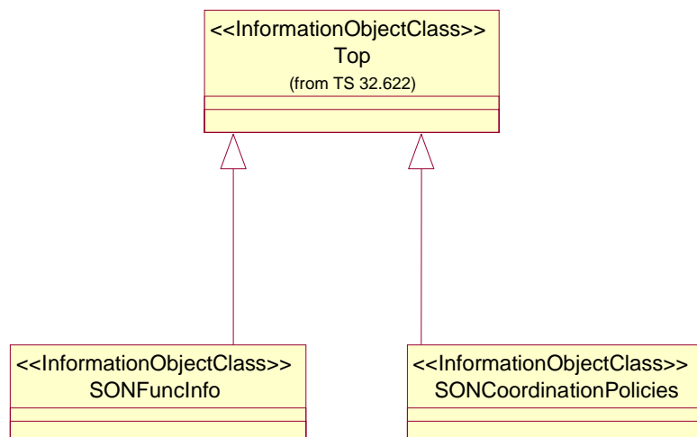
Figure 5.2.2-5: IOCs for SON coordination (Inheritance Relationship)
