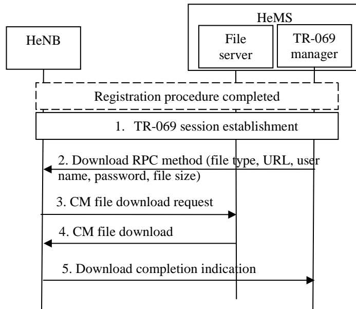
Figure 5-1 HeNB configuration using file download procedure
