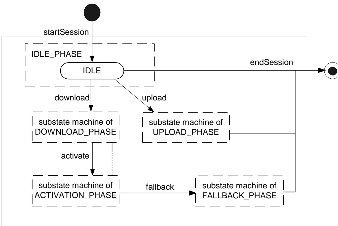
Figure 5: State Machine
