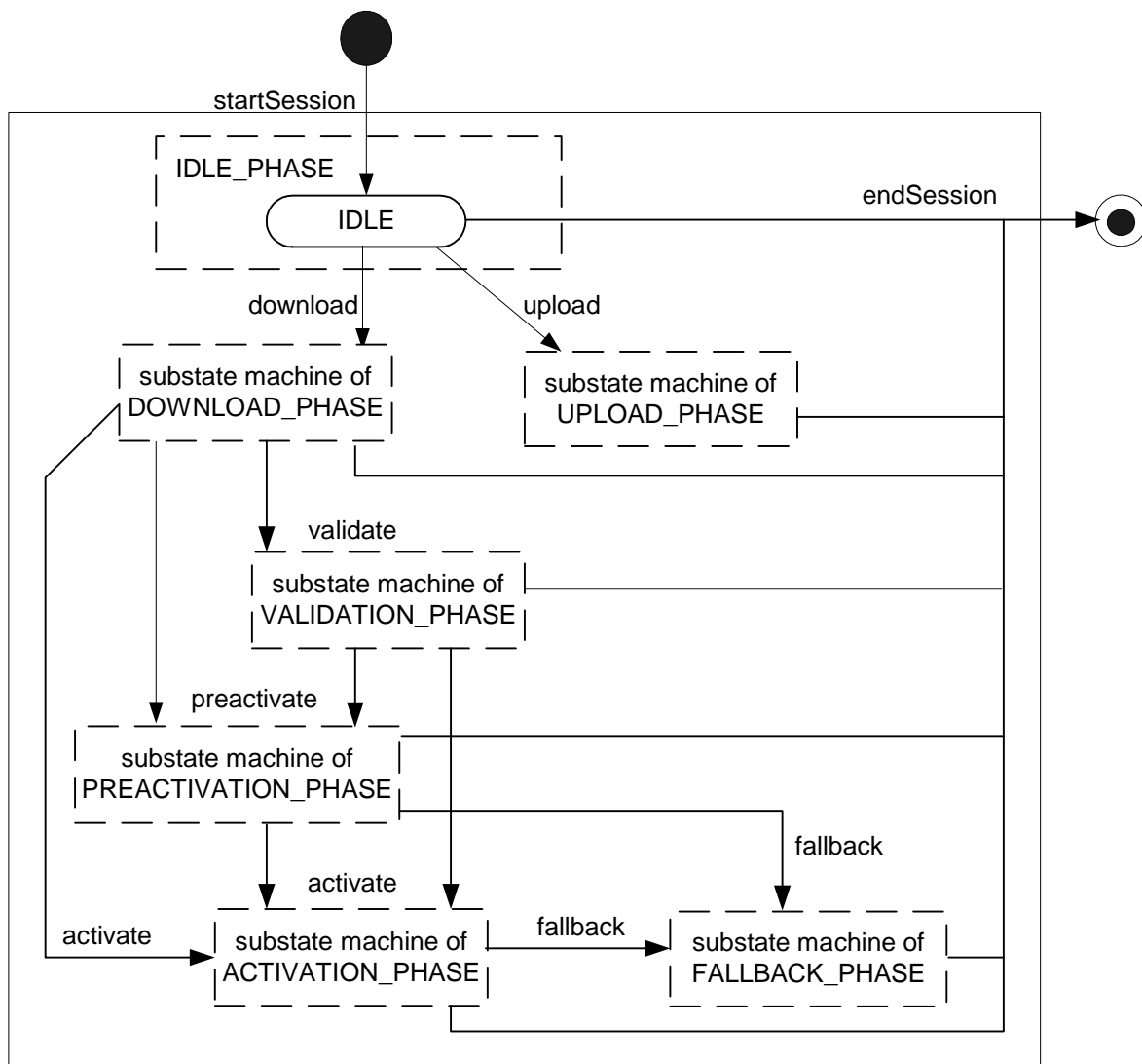
Figure : State Machine
