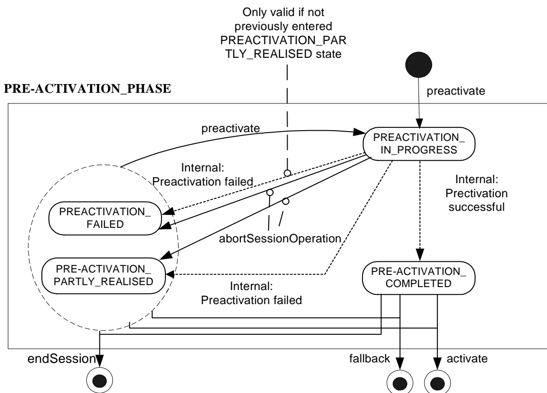
Figure : Substate Machine – PREACTIVATION_PHASE
