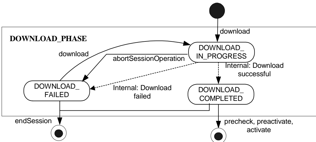
Figure : Substate Machine – DOWNLOAD_PHASE
