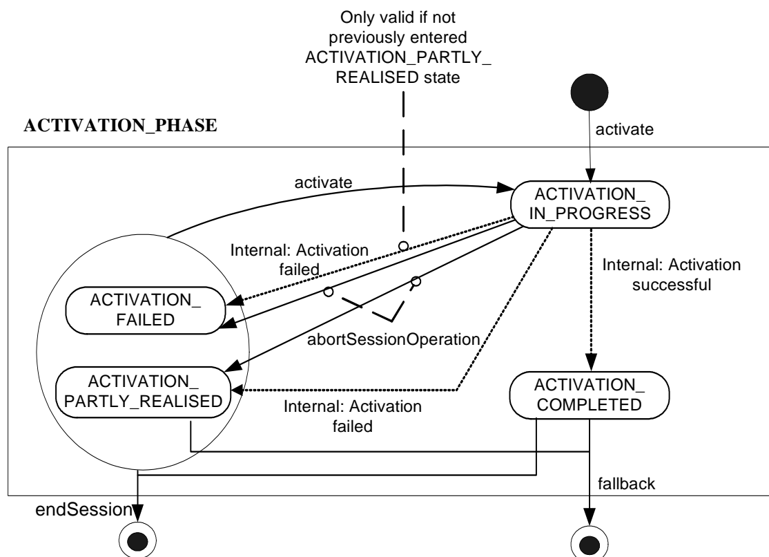
Figure 9.2.4: Substate Machine – ACTIVATION_PHASE
