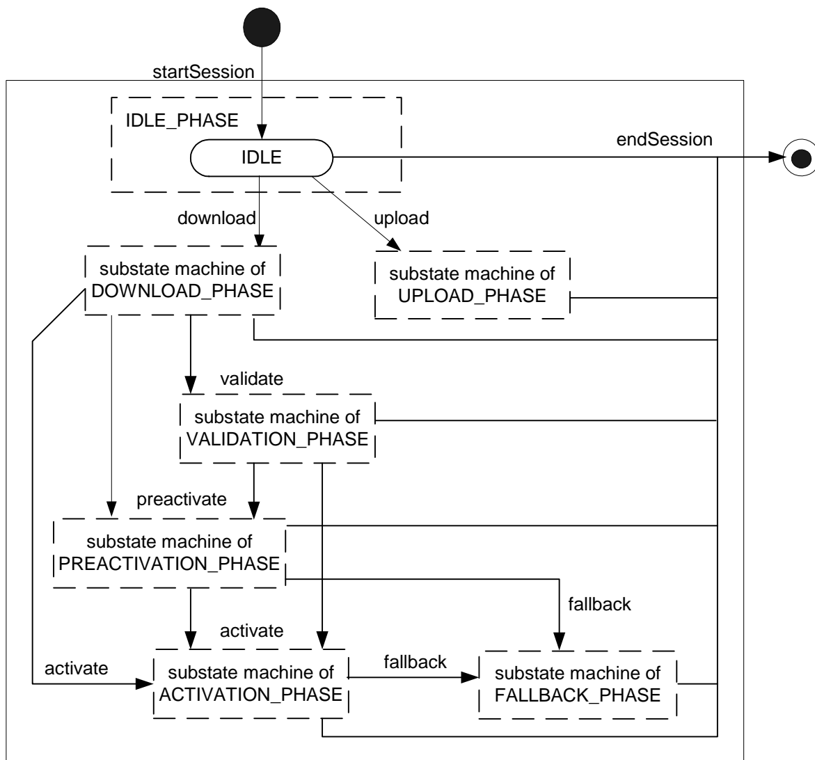
Figure 1: State Machine
