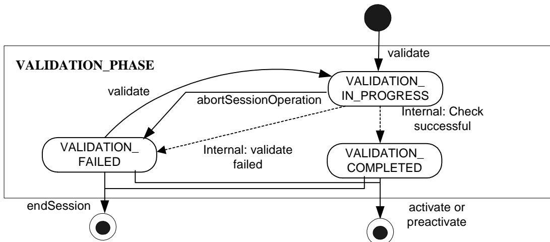
Figure 7: Substate Machine - VALIDATION_PHASE
