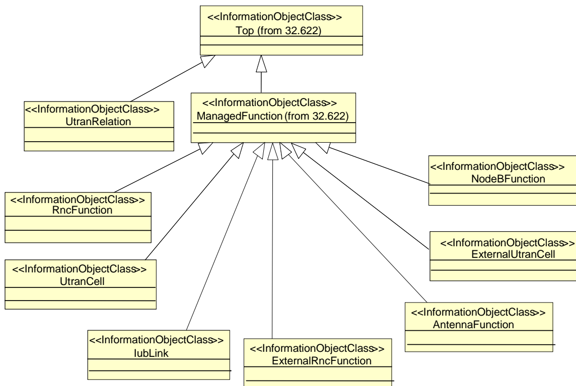
Figure 6.2.2.1: UTRAN NRM Inheritance Hierarchy
